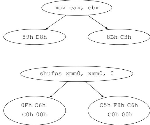
Fig. 2. Instruction semantics and their alternative encodings.
